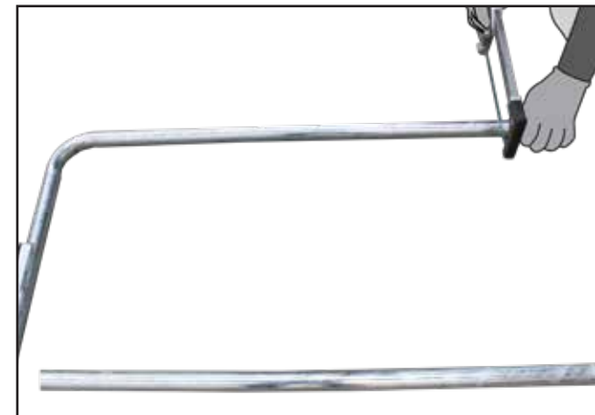
H. Using a hacksaw or similar, carefully cut through the top, bottom tubes, the toeboard and the mid rail as shown. For galvanised assemblies, spray with Galvafruid or similar to prevent corrosion.
