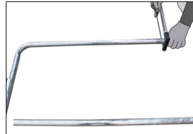
I. Using a hacksaw or similar, carefully cut through the top, bottom tubes, the toeboard and the mid rail as shown. For galvanised assemblies, spray with Galvafruid or similar to prevent corrosion.
